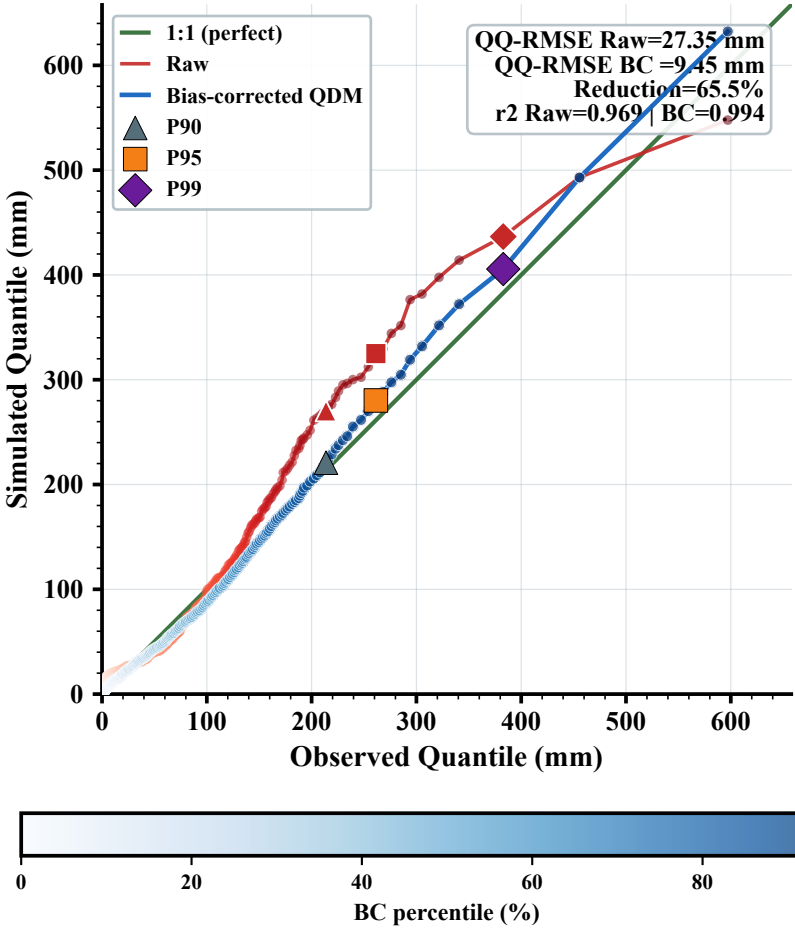
e MIROC6: Raw and BC vs Obs
