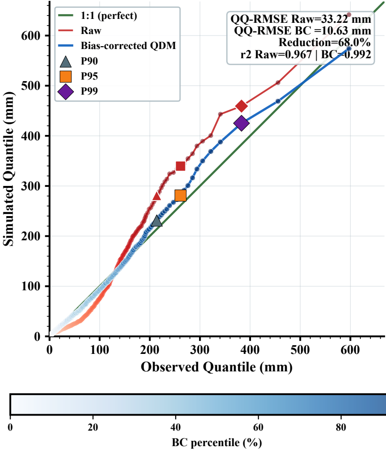
b CESM2: Raw and BC vs Obs
