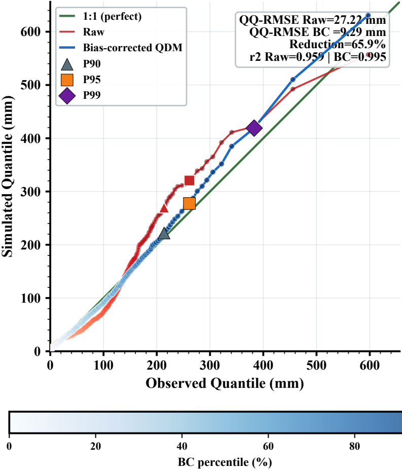
c CanESM5: Raw and BC vs Obs
