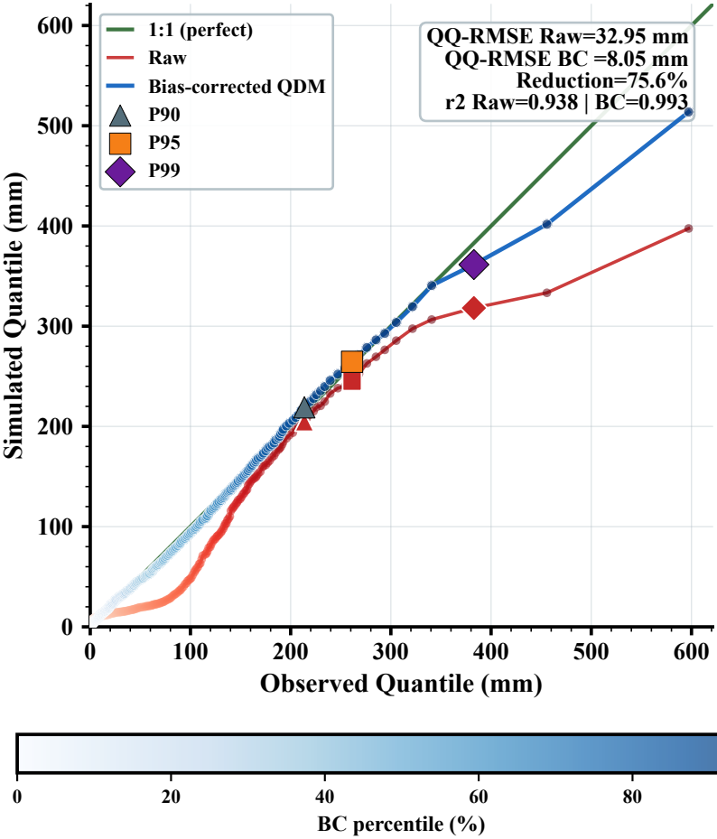
d EC-Earth3: Raw and BC vs Obs
