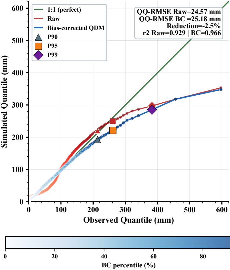
f Ensemble mean: Raw and BC vs Obs
