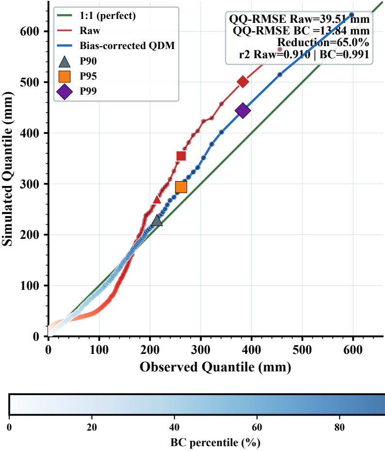
a ACCESS-ESM1-5: Raw and BC vs Obs
